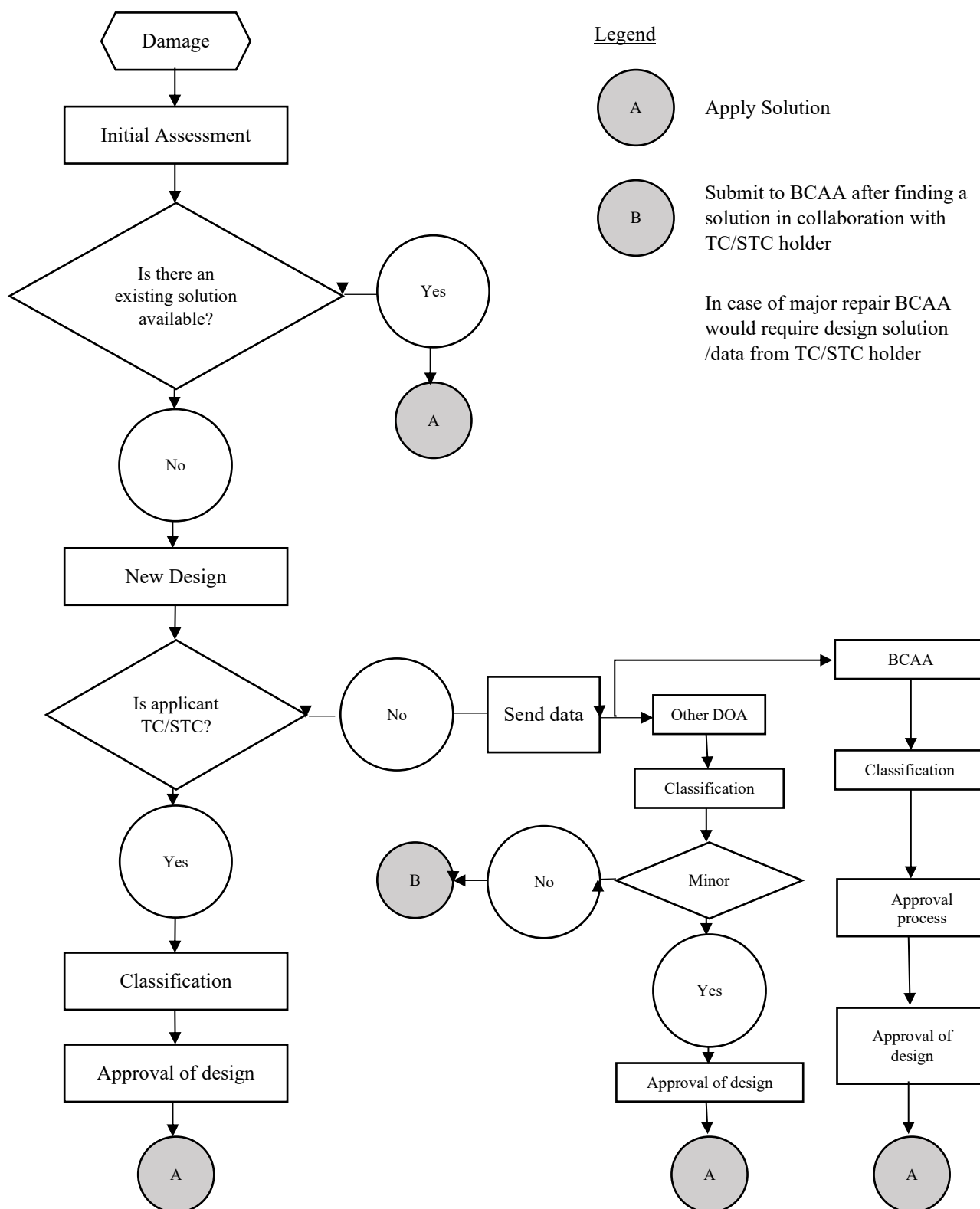
Flowchart 1 to GM 21.A.431(a) – Repair approval procedure
